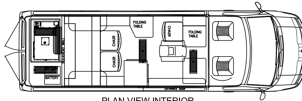
PLAN VIEW INTERIOR
