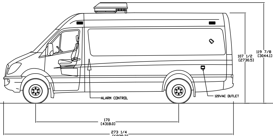
STREET SIDE EXTERIOR VIEW
