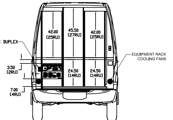
SECTION A-A INTERIOR RACK VIEW
