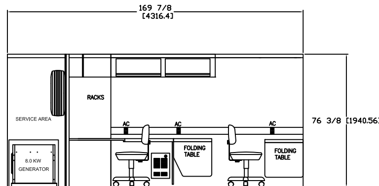
INTERIOR STREET WALL
