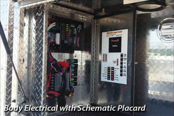
Intuitive Single Operator In-Cab Design
